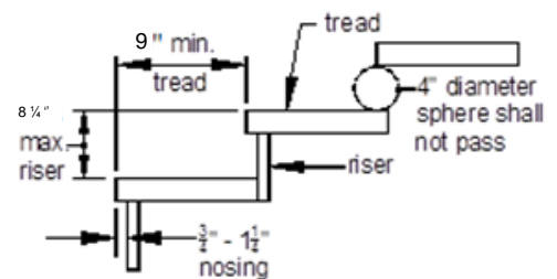
FIGURE 33: TREADS AND RISERS Worcester Amended
