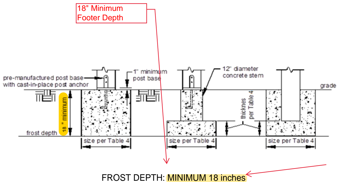
FIGURE 10: FOOTINGS
